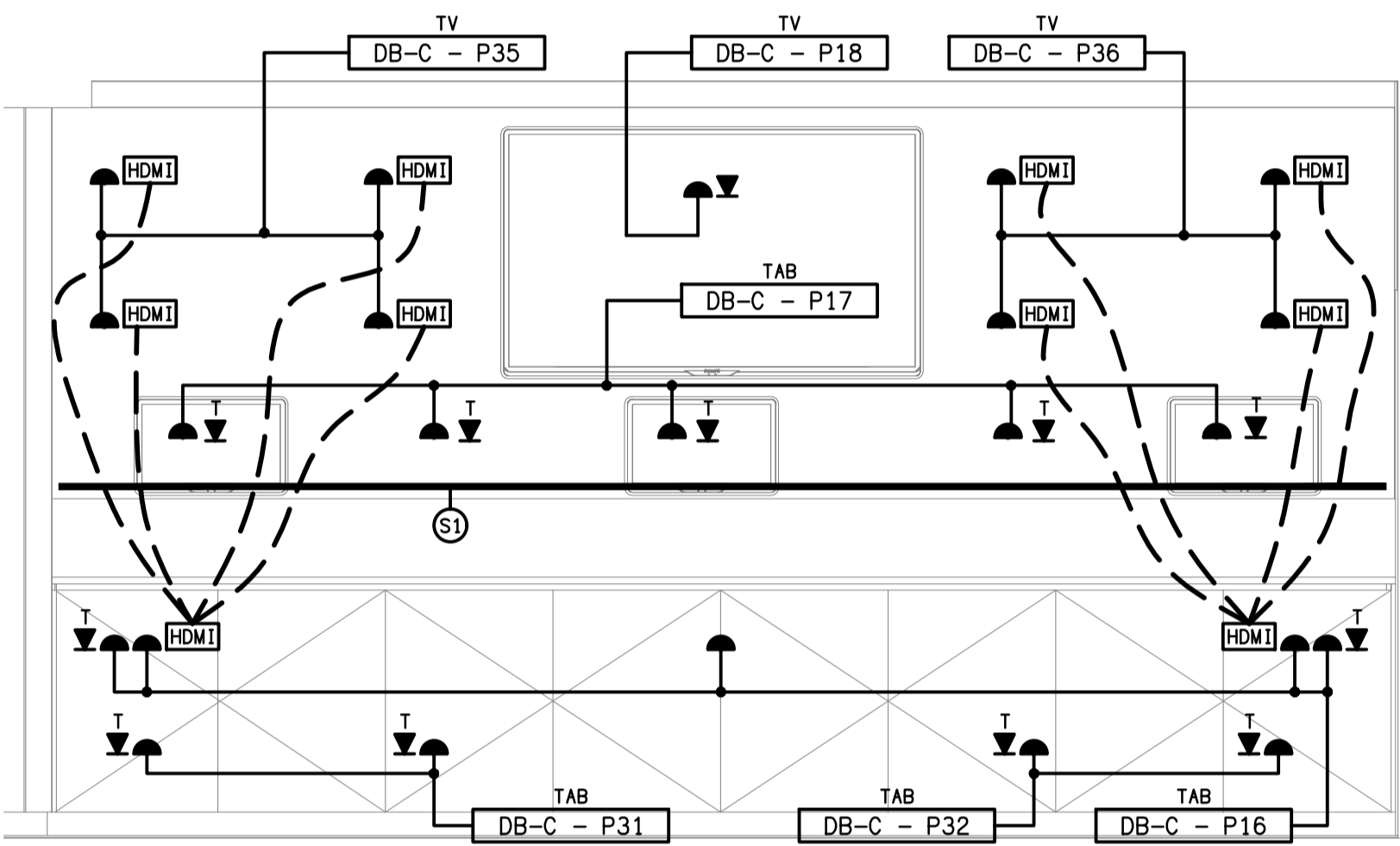
DETAIL A TAB WALL ELEVATION 1 SCALE 1:25
