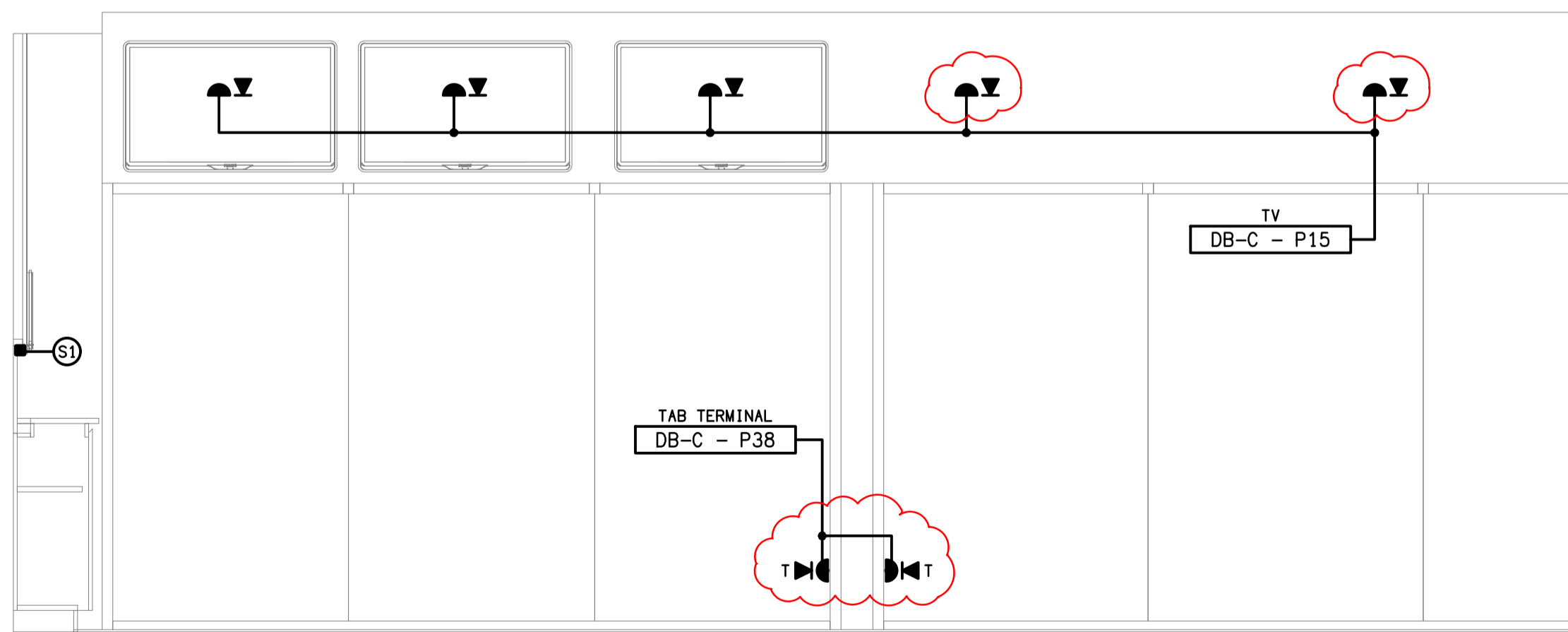
DETAIL B TAB WALL ELEVATION 2 SCALE 1:25
